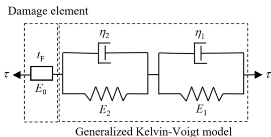
Fig. 14 Hybrid model for characterizing creep behavior of anchor–soil interface
