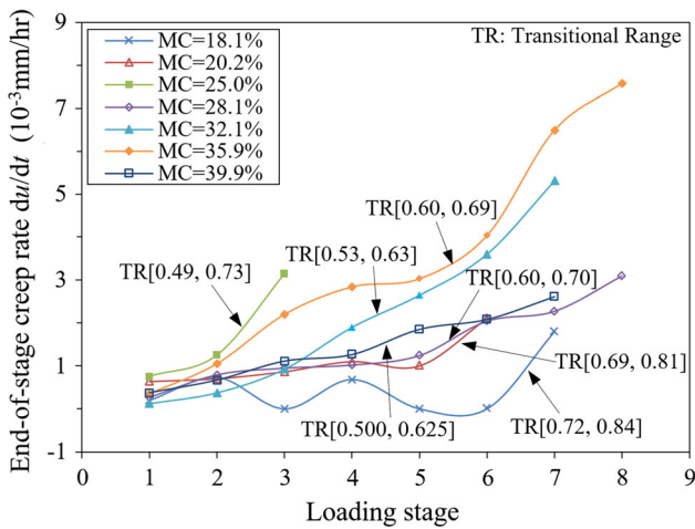
Fig. 12 End-of-stage creep rate with increasing loading stages for specimens with varying moisture conditions
